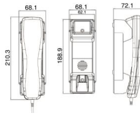
HANDSET
